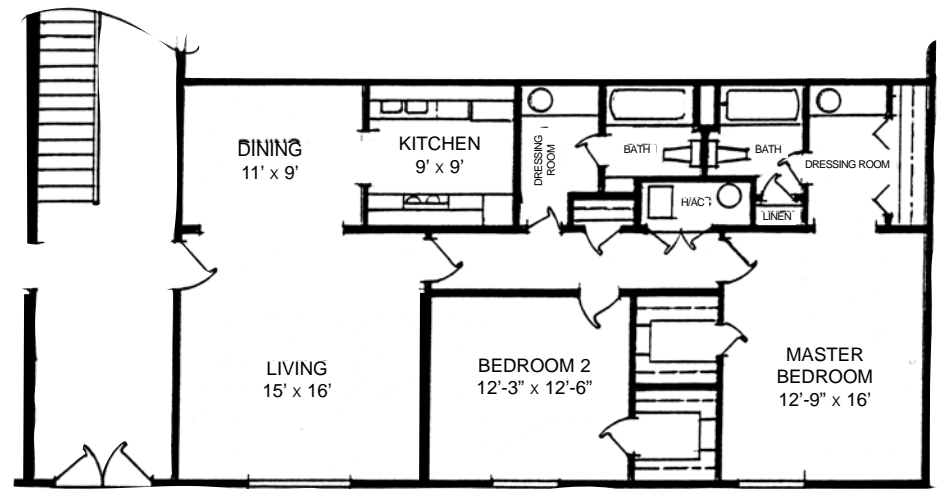
TWO BEDROOMS TWO BATH WITHS DRESSING ROOMS 1300 SQUARE FEET
